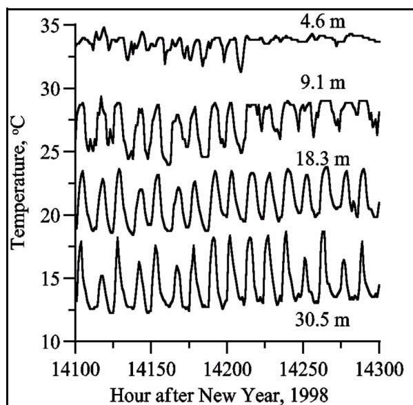
Figure 5. Original temperature records for four depths at WIES, Santa Catalina Island, 11–19 August 1999. All traces except the 30.5-m depth are offset from adjacent ones by 5^{\circ}\text{C} .
