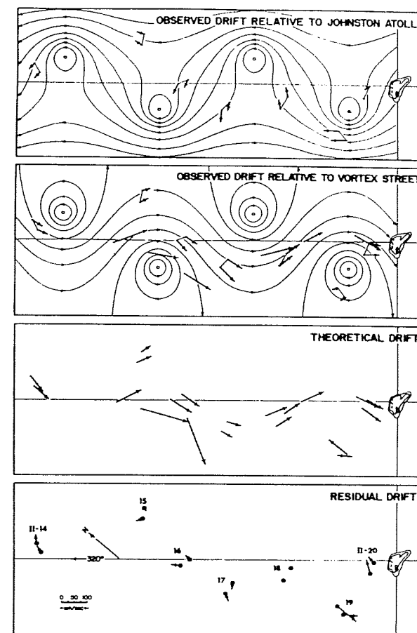
FIGURE 1. Eddies in the wake of Johnston Atoll (Barkley 1972, fig. 3). Streamlines were derived from von Kármán vortex street model fitted to direct current measurements (arrows). Degree of success of the model is evident from comparison of the two lower panels.
