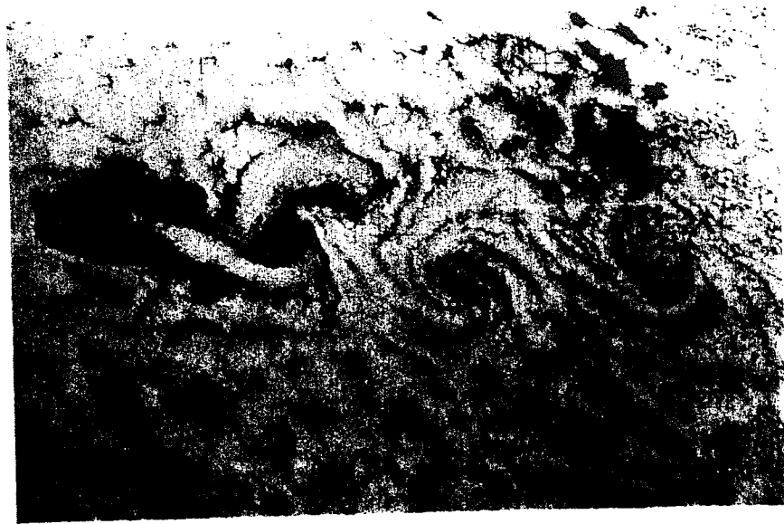
FIGURE 4. Vortices in the atmospheric wake of Guadalupe Island off Baja California from Skylab on 6 September 1973 (NASA photograph SL-3 #121-2371).
