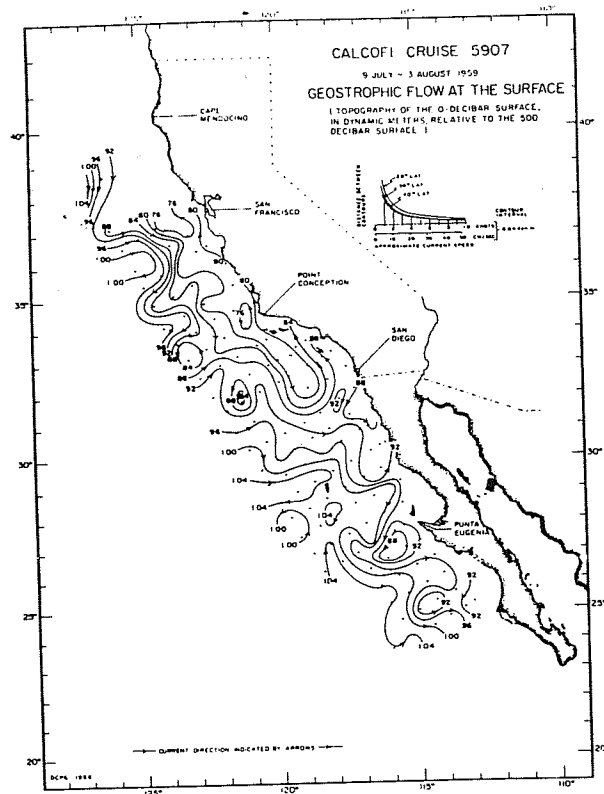
FIGURE 7. Baroclinic representation of surface flow off the Californias in July 1959 (Wyllie 1966, p. 124). Eddies large enough to deform the density field and to be detected by the sampling grid (dots) appear as closed isobars; meanders appear as loops.
