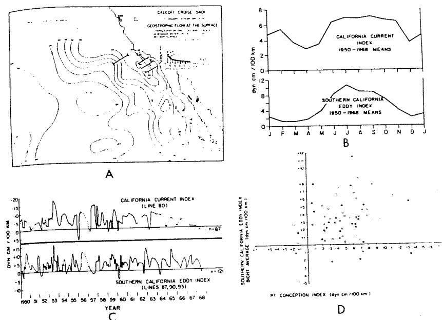
FIGURE 12. Indices of baroclinic flow across sections (Panel A) off Point Conception (Panel B and C upper) and in the SC Eddy (Panel B and C lower), and the relationship between individual index pairs (Panel D). Indices derived from Wyllie (1966) by the author.
