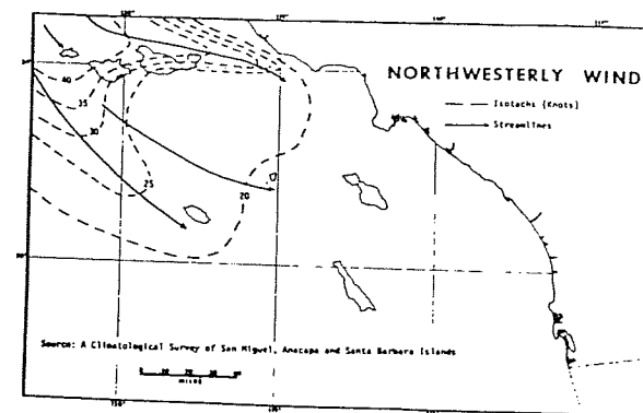
FIGURE 3. Wind speed and direction over the SC Bight during northwest winds (U.S. Dept. Interior 1978, p. 65).
